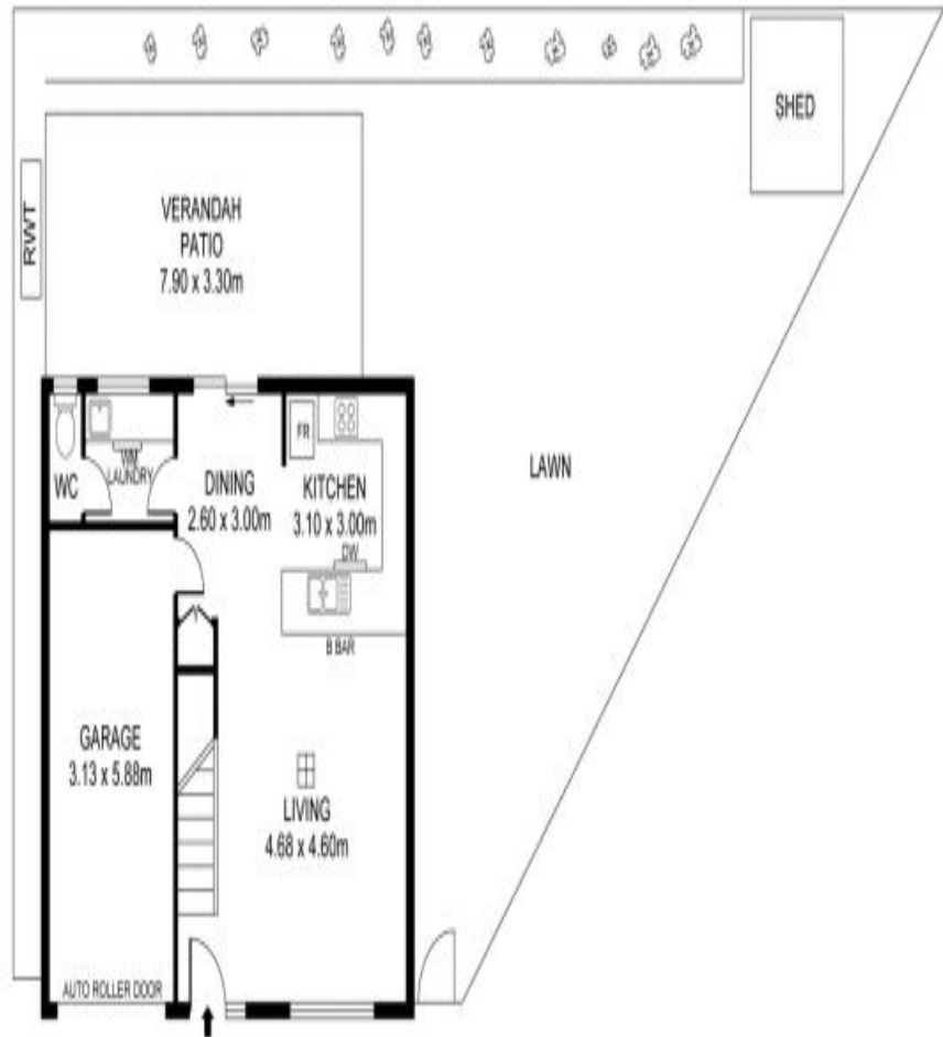
GROUND FLOOR - 68 SQM
